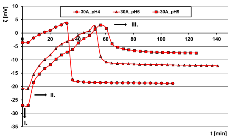
Figure 4: Standard polyester fabric 30A as adsorbent and desorbent in the electrokinetic system SurPASS in phase I, phase II and phase III
