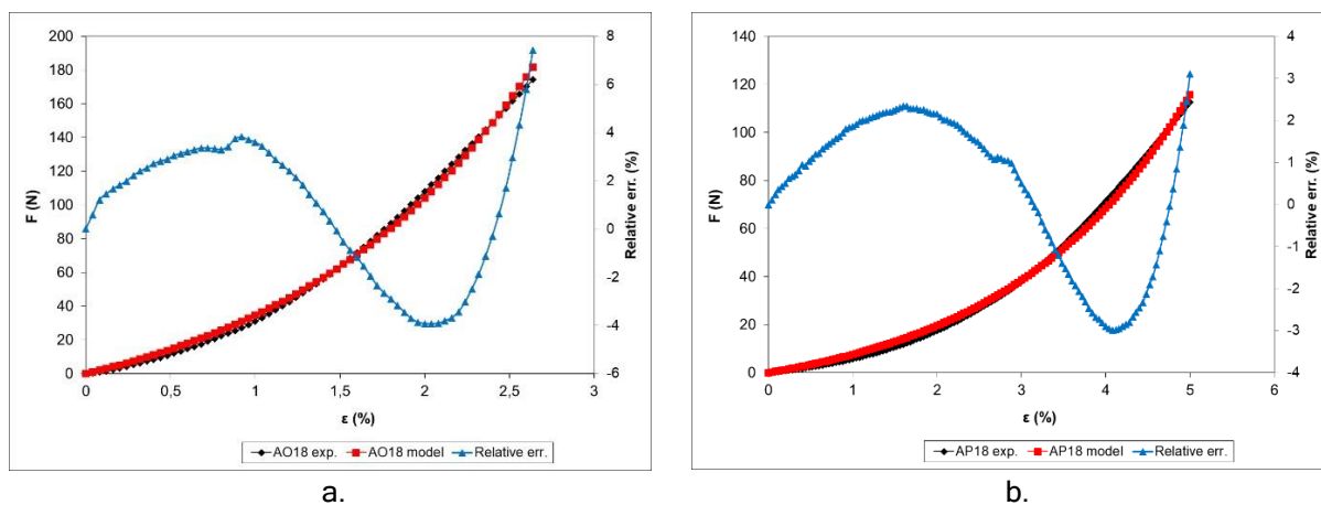
Figure 5: Diagram force-elongation (F- \epsilon ) obtained experimentally and by model: a) sample AO18, b) sample AP18
