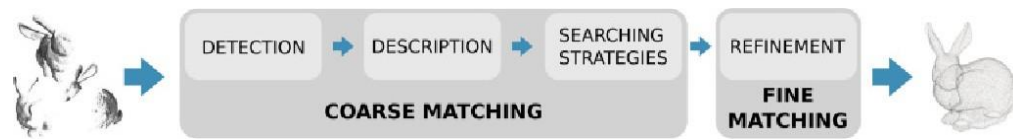
Figure 2: Pipeline of the detection-description-matching approach. Taken from [13].
