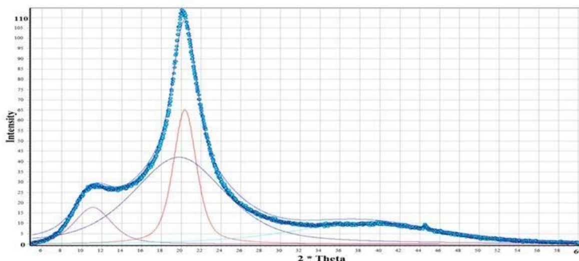
Figure 3: Sample ID 1.4, WAXS curve resolved into crystalline peaks (red curve) and amorphous (blue, thin curve) components. On the graphic plot it can be observed that the Chitosan's characteristic crystalline peaks at maximum are located at 2\theta=21^\circ and amorphous halos from chitosan are present from 2\theta=0^\circ to 40^\circ .
