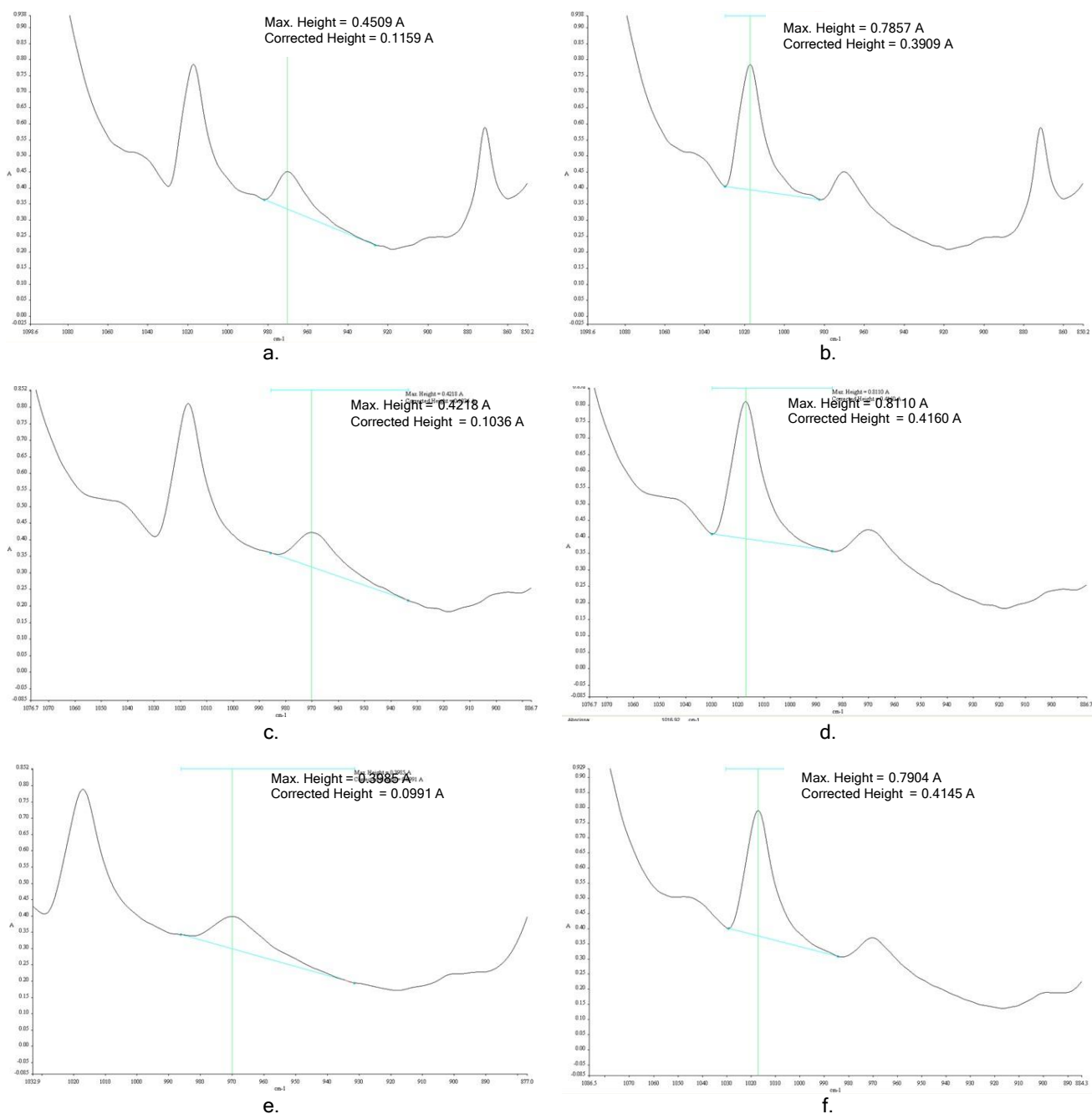
Figure 2: The characteristic FT-IR absorption band at wavelengths 970 cm -1 (a, c, e) and 1017 cm -1 (b, d, f) of untreated PET (a, b), alkali hydrolysed PES-H (c, d) and lipase hydrolysed PES-L (e, f) fabrics
