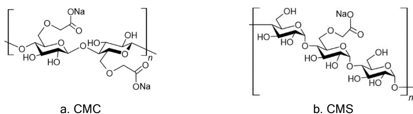
Figure 1: Chemical structure: a. carboxymethyl cellulose (CMC) [7], b. carboxymethyl starch (CMS) [8]
