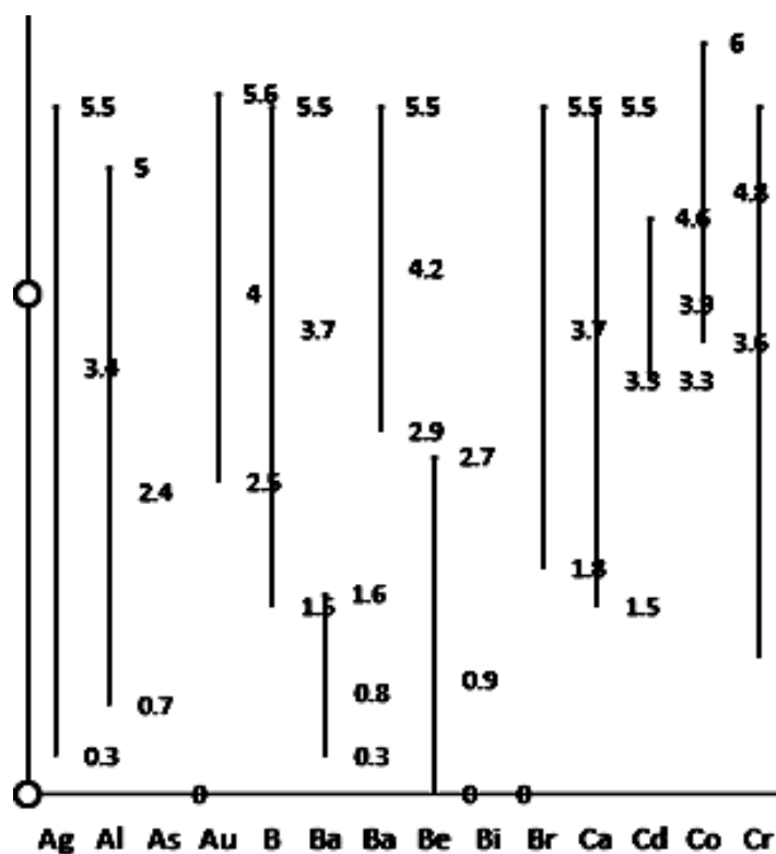
Figure 1: Spot position, width and overlapping of investigated metal ions: Ag + , Al 3+ , As 2+ , Au 2+ , B + , Ba 2+ , Be 2+ , Bi 3+ , Br - , Ca 2+ , Cd 2+ , Co 2+ and Cr 3+ detected on Cellulose F , producer KEMIKA, precoated plates, developed under optimal conditions under the front distance of 8 cm
