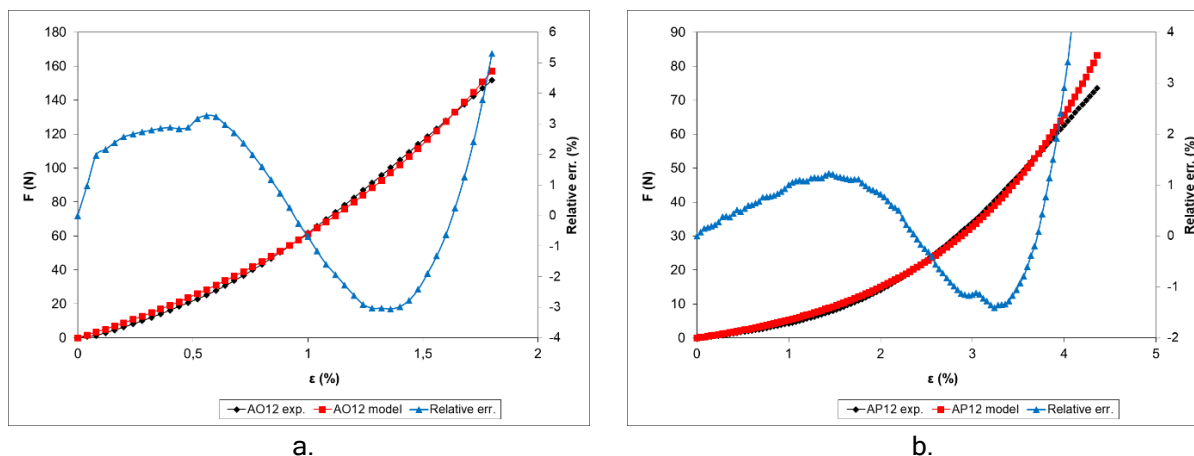
Figure 4: Diagram force-elongation (F- \varepsilon ) obtained experimentally and by model: a) sample AO12, b) sample AP12
