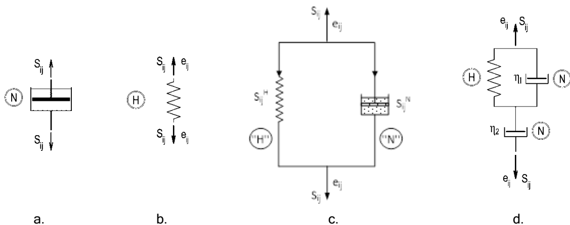
Figure 2: Rheological models: a) Newton's model, b) Hooke's model, c) Kelvin's model, d) Lethersich's model
