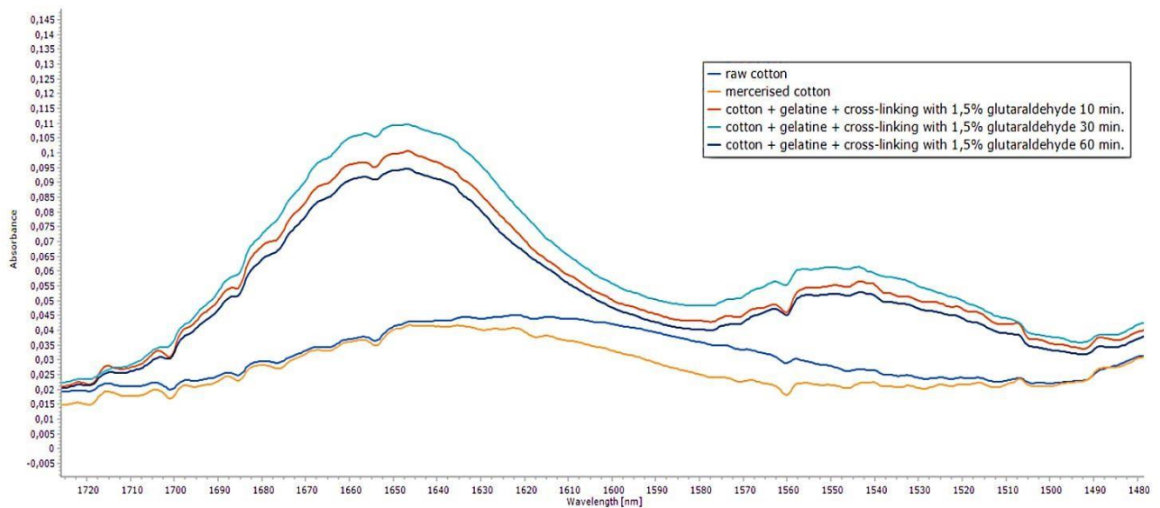
Figure 6: FTIR spectrum for cotton fabric modified with gelatine crosslinked with 1.5 % glutaraldehyde..
