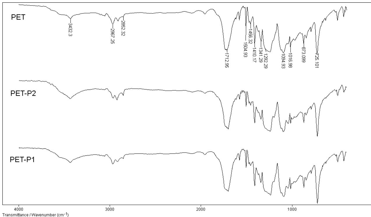
Figure 1: FTIR diagram of PET and PET-treated samples
