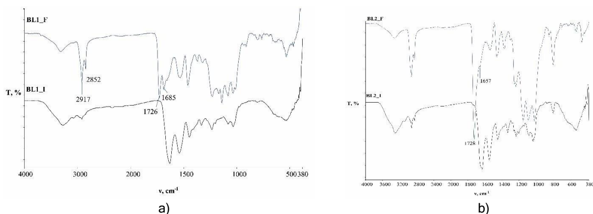
Figure 1: FT-IR spectrum curves of BL1 (a) and BL2 (b)
