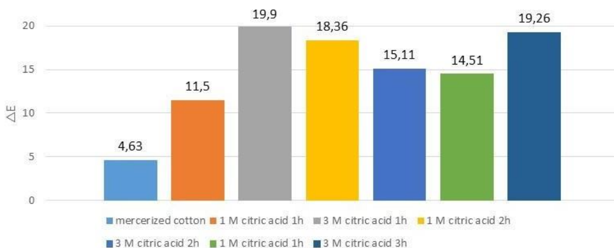
Figure 4: \Delta E values for samples modified with grafted gelatine and citric acid.
