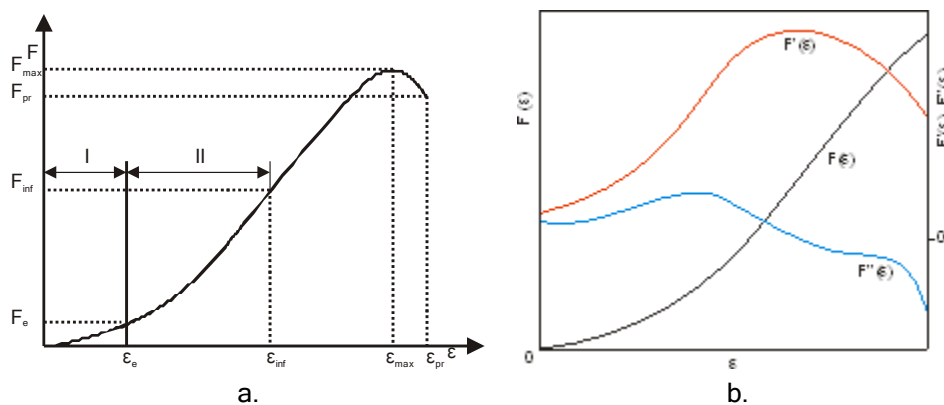
Figure 1: Dependency diagram force-elongation: a) the characteristic diagram of force - elongation ( F - \epsilon ) of the woven fabric, b) the function F(\epsilon) , the first F'(\epsilon) and the second F''(\epsilon) derivation of the function
