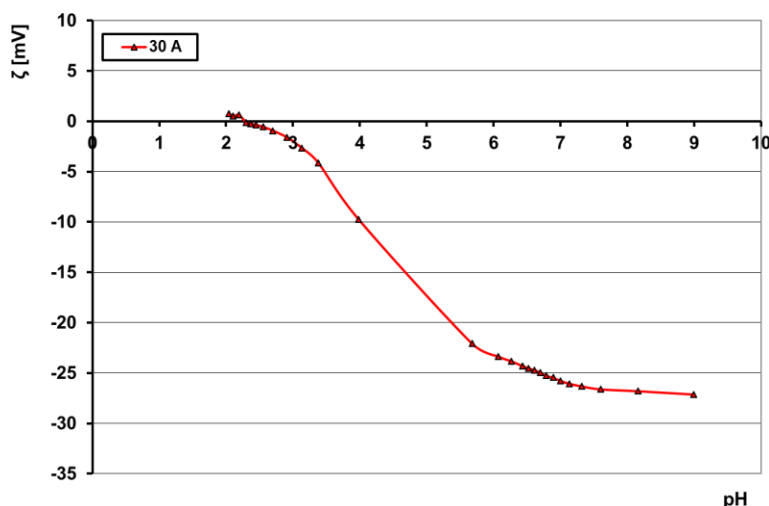
Figure 3: Zeta potential of standard polyester fabric (30A) in variation of pH of a 1 mmol/L KCl
