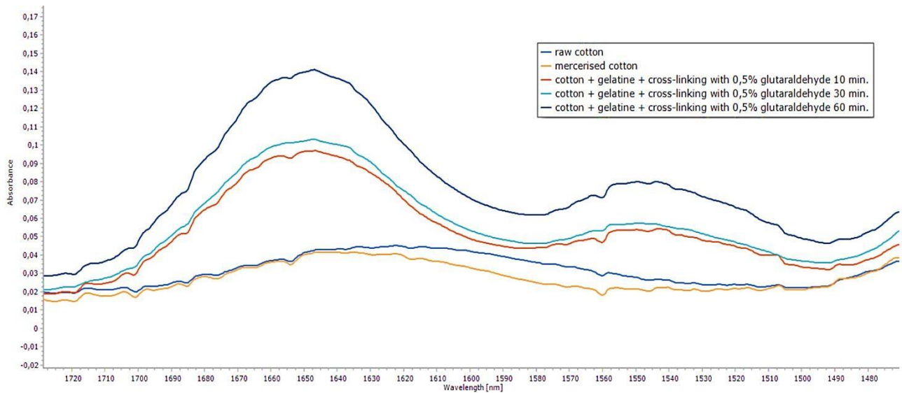
Figure 5: FTIR spectrum for cotton fabric modified with gelatine crosslinked with 0.5 % glutaraldehyde.
