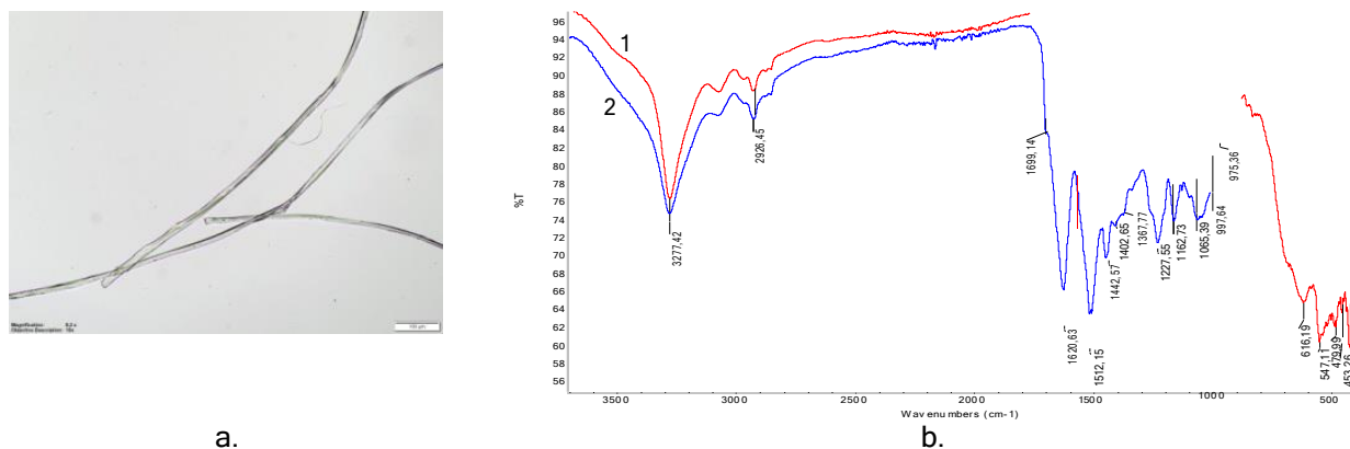
Figure 5: Previous repairs performed with a thread in beige color: a. longitudinal microscopic image of the fiber, b. FTIR comparison: sample of thread used in repair (2) and referent spectra of silk fiber (1)
