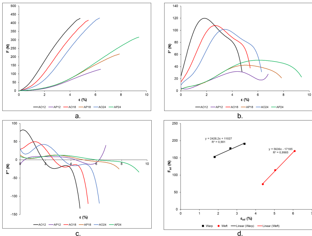
Figure 3: Diagrams for samples with different weft densities: a) force - elongation ( F-\epsilon ), b) the first derivation of a function F'(\epsilon) , c) the second derivation of function F''(\epsilon) , d) force F_{\text{inf}} - elongation \epsilon_{\text{inf}} at the inflection point
