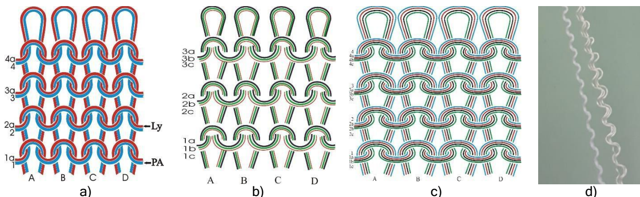
Figure 1: Plated jersey structures used in the manufacturing of plain socks; a) plain plated structure - two yarns in a row, b) multiple plated structure - three threads in a row, c) multiple plated structure - four yarns in a row, d) four separated yarns from a row; PA – cotton, Ly - elastane
