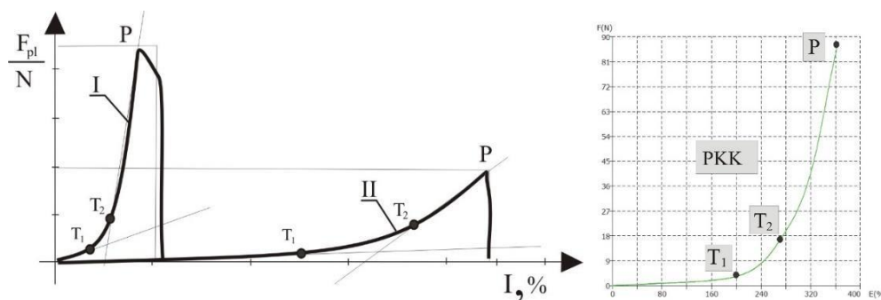
Figure 3: Force/extension diagrams for double jersey weft knitted fabric: a) extension diagrams of the knitted fabric in the wale direction (I) and in the course direction (II); T1 - end of the elastic region, T2 – point of the onset of plastic deformation, P – point of knitted fabric breakage, b) extension diagram of the knitted fabric in the course direction, knitted fabric made of a 20 tex yarn
