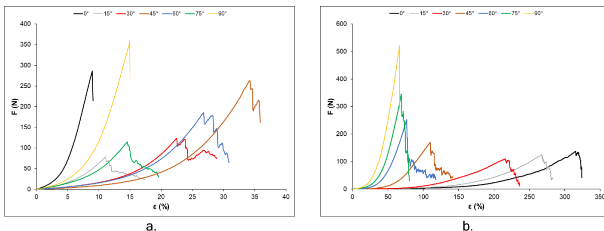
Figure 2: Diagram force - elongation ( F - \varepsilon ): a) woven fabric sample, b) knitted fabric sample
