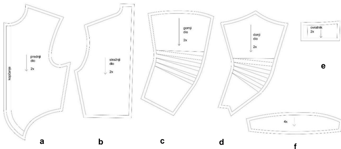
Figure 2: Modeled patterns of the garment: a) front, b) back, c) upper sleeve, d) lower sleeve, e) collar, f) crescent-shaped insert
